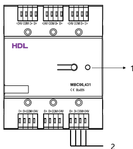
Figure 4. Components - Front View
