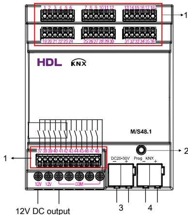
Figure 4. Wiring
